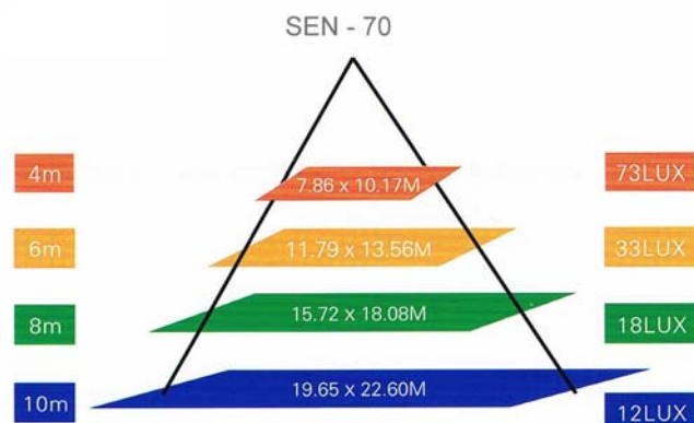
Isolux diagram
