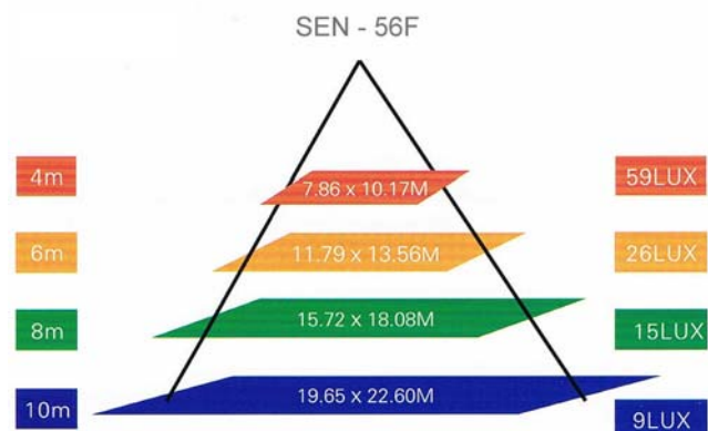
Isolux diagram
